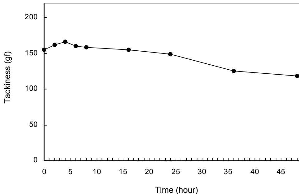
Tackiness Data
